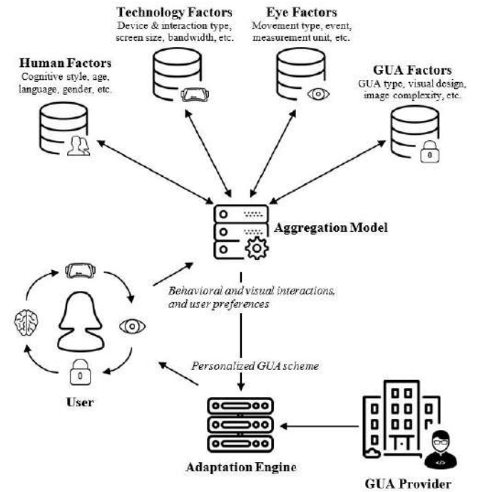
Figure 7: Conceptual design of an extensible framework specialized in delivering personalized GUA schemes
